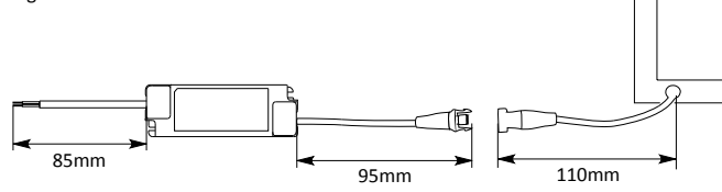
Fig. 1. Cables dimensions.
