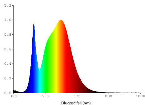
LEDSTAR ECO A60, 9W, NB - 4000K
